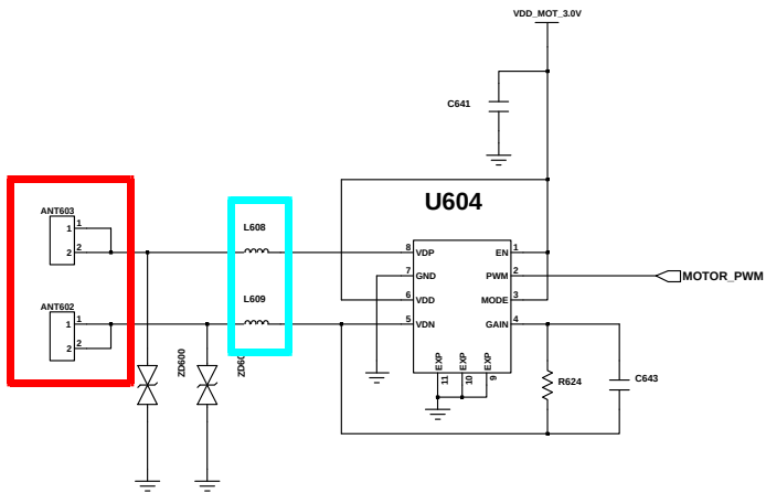
Haptic Driver
